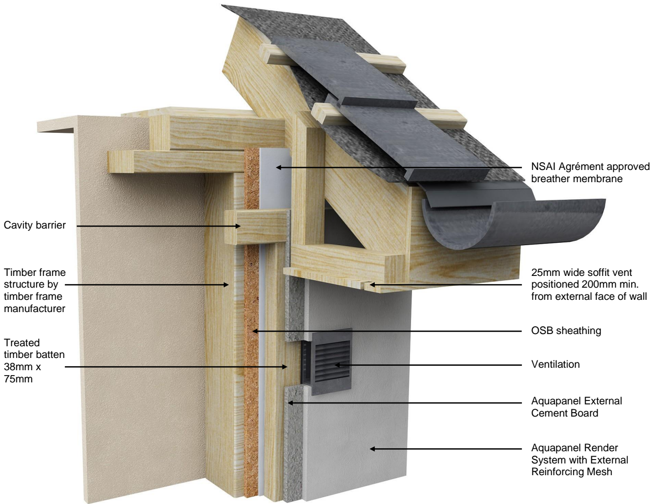
Figure 6: Eaves detail
