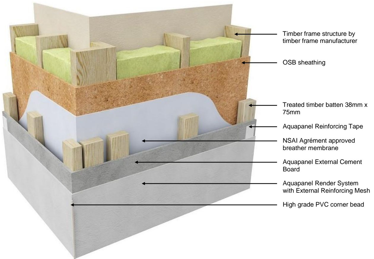
Figure 7: Corner detail
