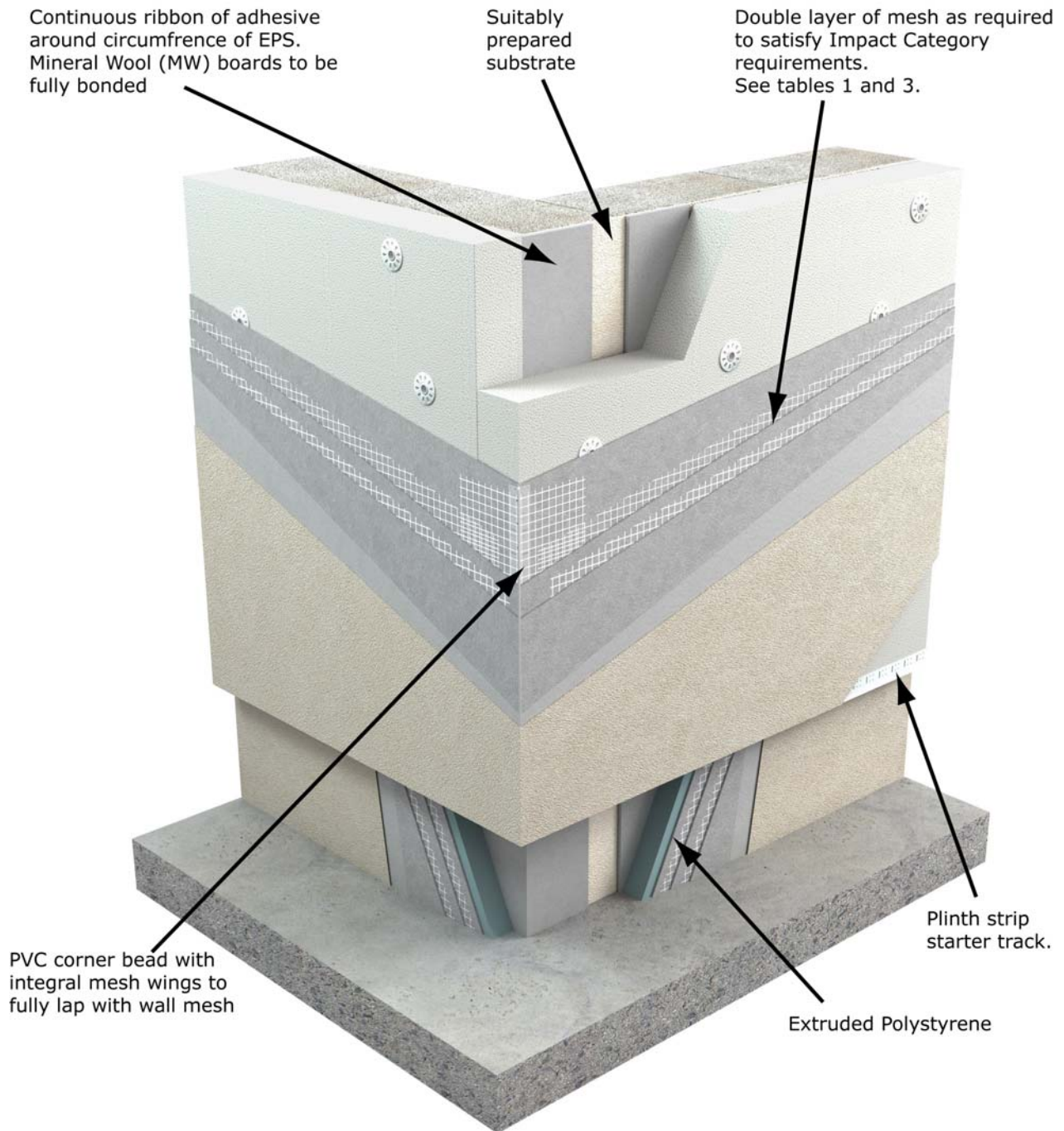
Figure 1: Corner/Plinth/Wall Details
